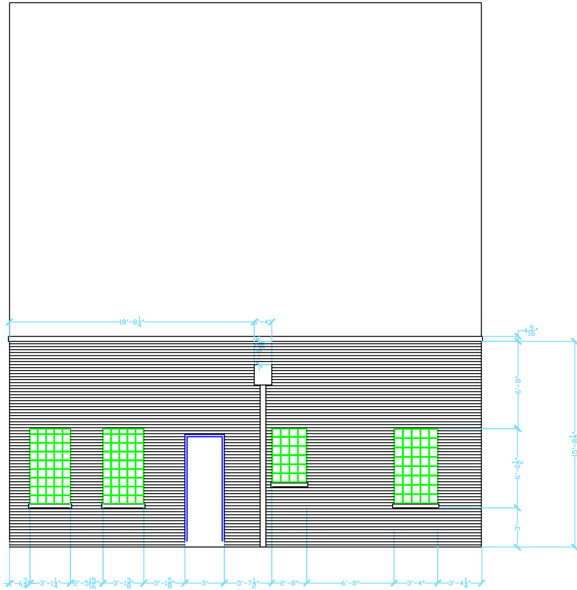
SOUTH EXTERIOR
